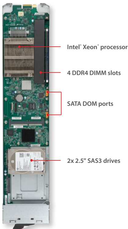
Figure 5. 1 of 14 hot-swap MBL-6119G-C2 Server Blades
